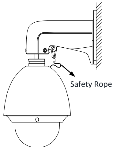
Figure 2-6 Safety Rope
