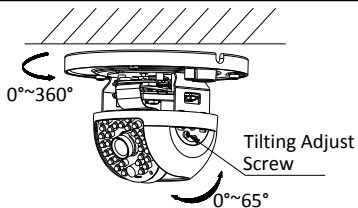
Figure 2-6 Angle Adjustment of Type I Camera
