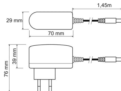
Fig.1. Dimensions of power supply.
