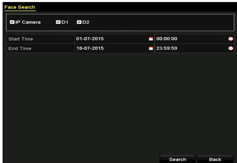
Figure 11-1 Face Search
