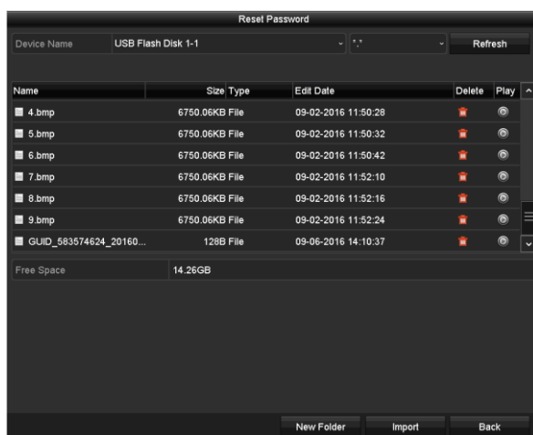
Figure 2-31 Import GUID
