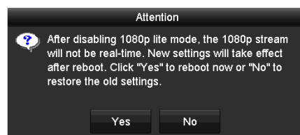
Figure 5-47 Attention
