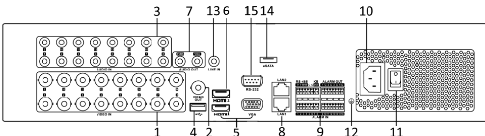
Figure 1-21 Rear Panel of DS-9000HUHI-F8/N
