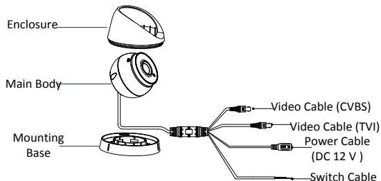
Figure 1. 5 Overview of Type V Camera
