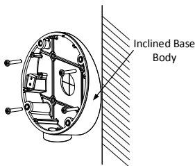
Figure 2. 30 Fix the Inclined Base Body
