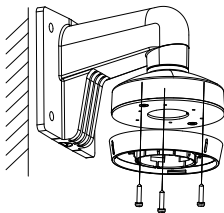
Figure 2. 27 Attach the Mounting Base to the Bracket
