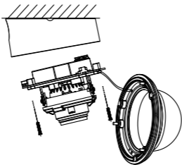
Figure 2. 12 Fix the Camera to the Base
