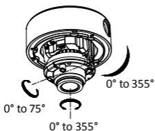
Figure 2. 4 3-Axis Adjustment
