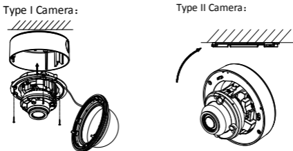
Figure 2. 3 Fix the camera to the Ceiling
