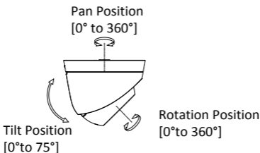
Figure 2-23 3-axis Adjustment
