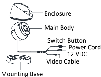
Figure 1-1 Overview of Type I Camera
