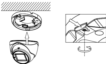
Figure 2-10 Install the Turret Camera
