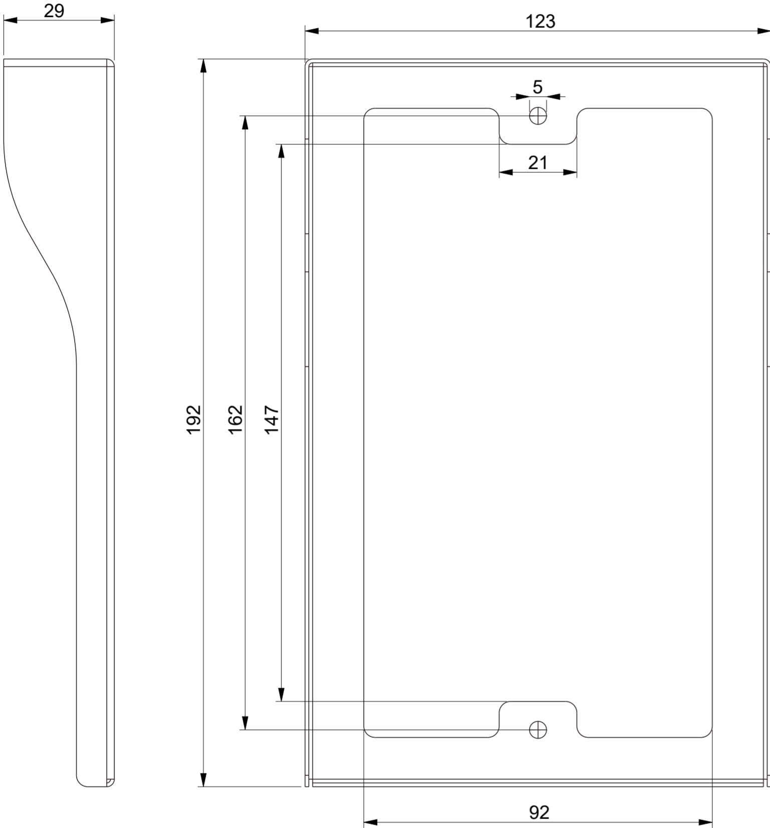
1 FRONT VIEW
