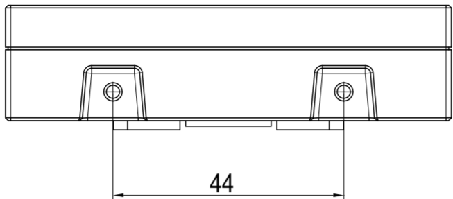
6 BOTTOM VIEW
