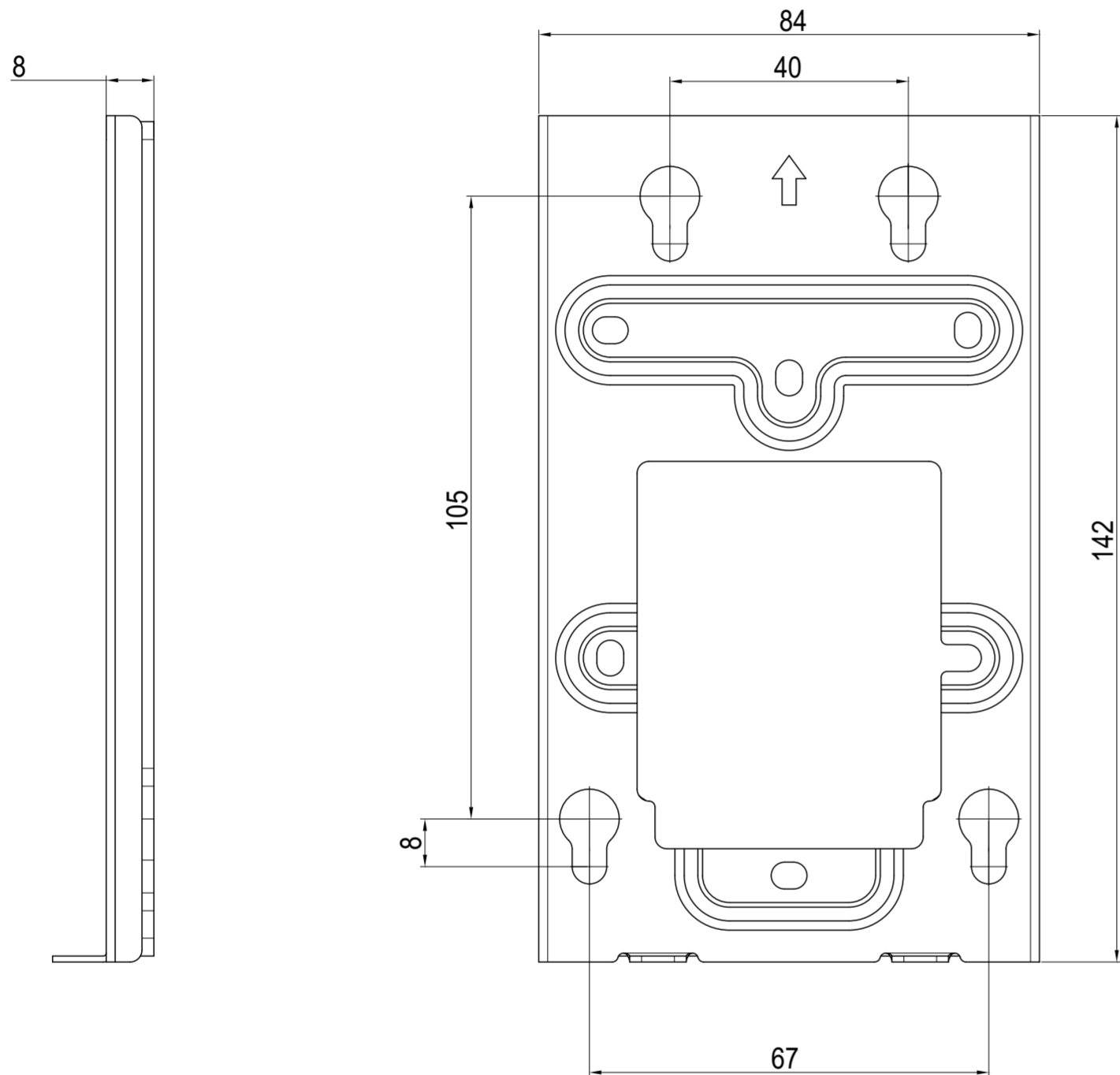
1 FRONT VIEW
