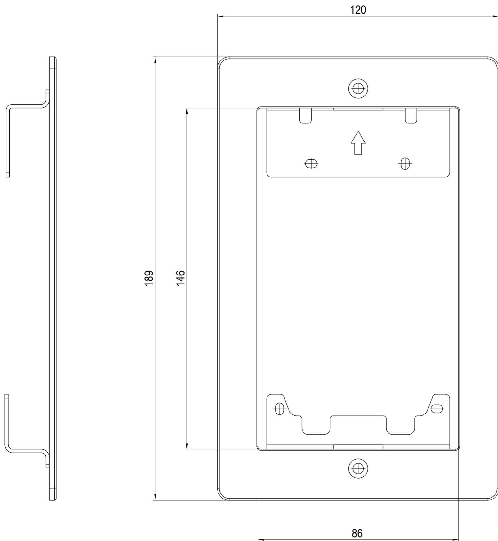
1 FRONT VIEW
